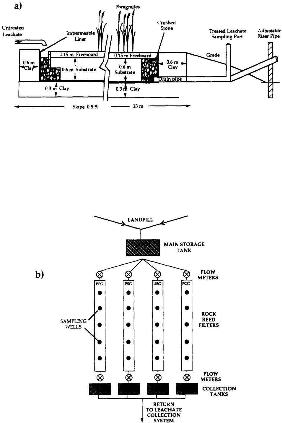
Fig. 1. (a) Schematic cross-sectional view of a rock-reed filter. (b) Plan view of the field layout. PCG = planted coarse gravel; USG = unplanted sand and gravel; PSG = planted sand and gravel; PPG = planted pea gravel.
